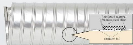
HEAT RESISTANT DUCT HOSE
